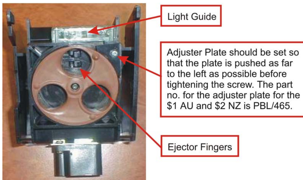
Figure 4: Serviceable Parts
